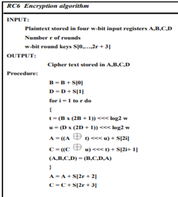
Fig 6: Encryption algorithm of RC6
