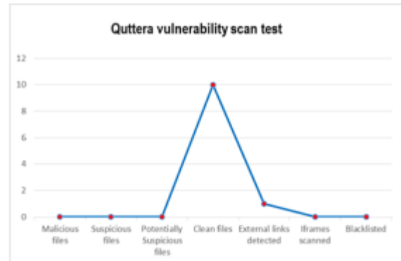
Fig 12: Qattara Vulnerability Testing Result
